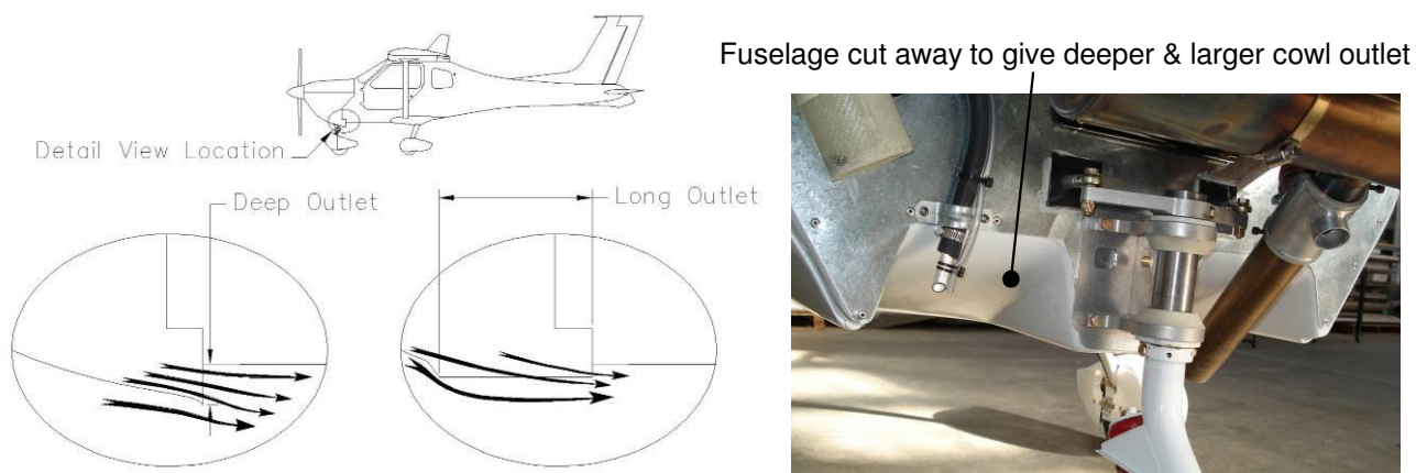
Figure 58. Cowl Outlet Geometry
