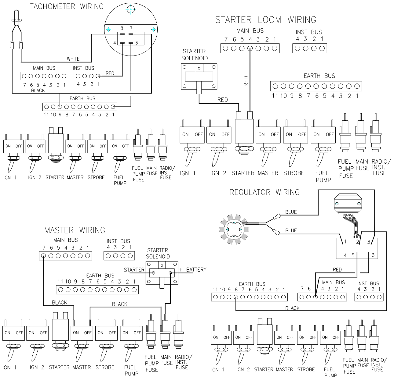
Figure 63. Wiring Details
