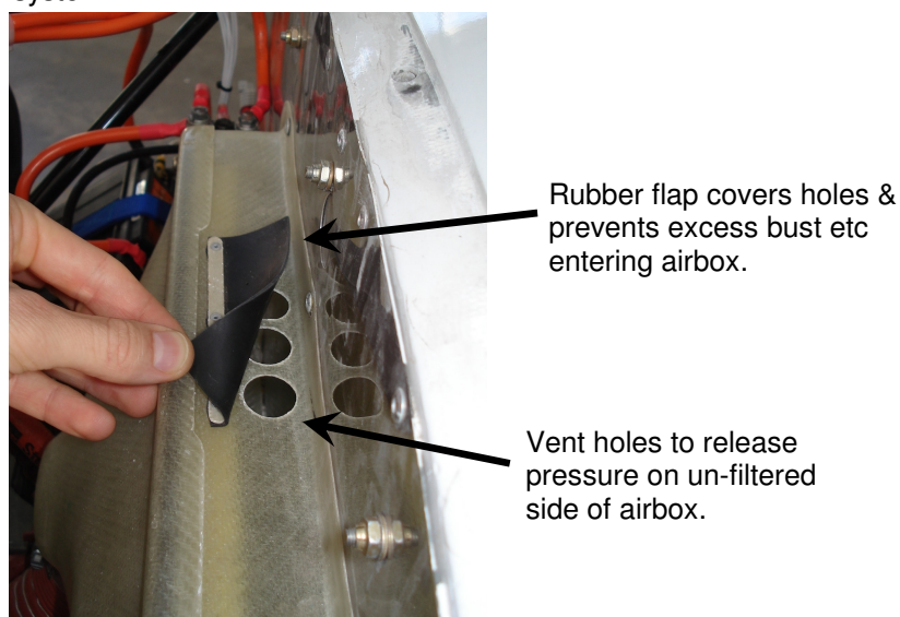
Figure 38. Ram Air Bleed
