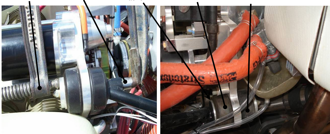
Figure 41 Upper & Lower Engine Mount Detail
