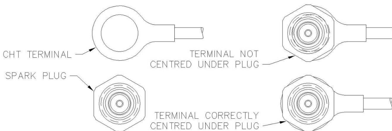
Figure 23. CHT Terminal Installation
