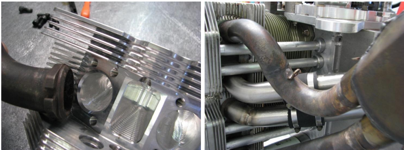
Figure 188 – Exhaust Installation
