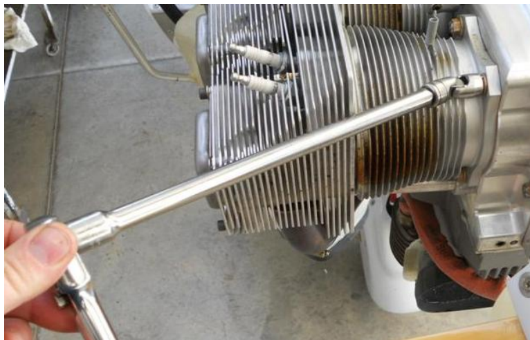
Figure 157 – Universal Joint tool FU14B (FU16B for 1/2" Socket)
