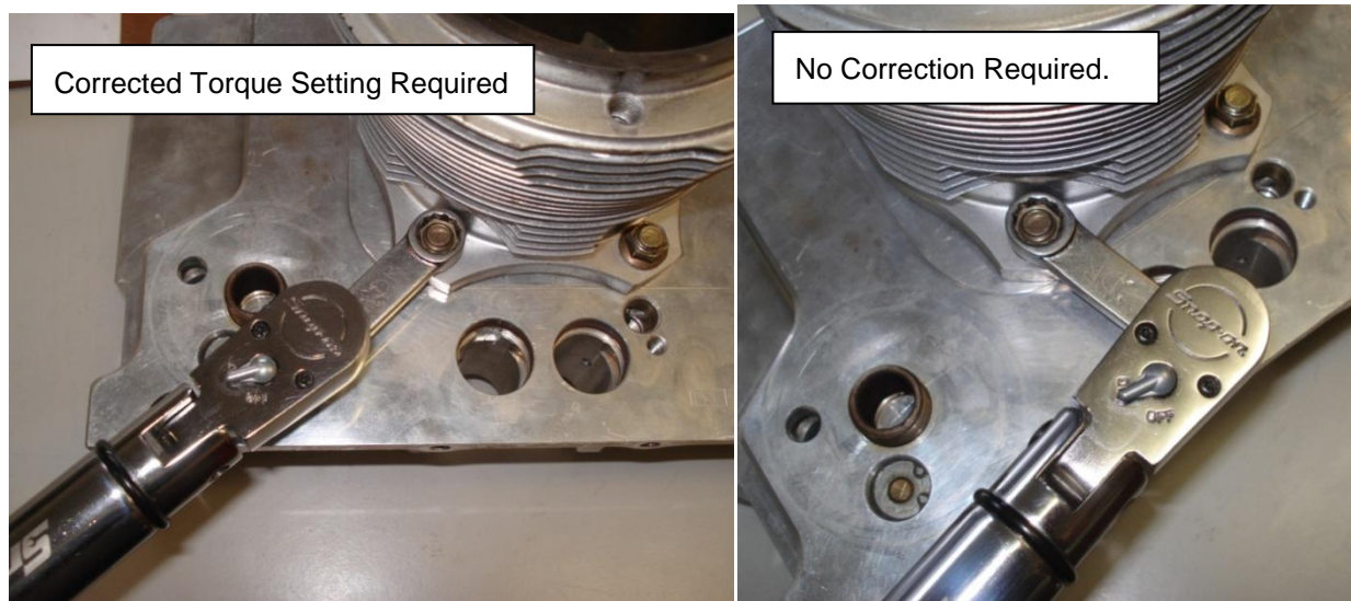
Figure 41 – Using A Crowsfoot Adaptor
