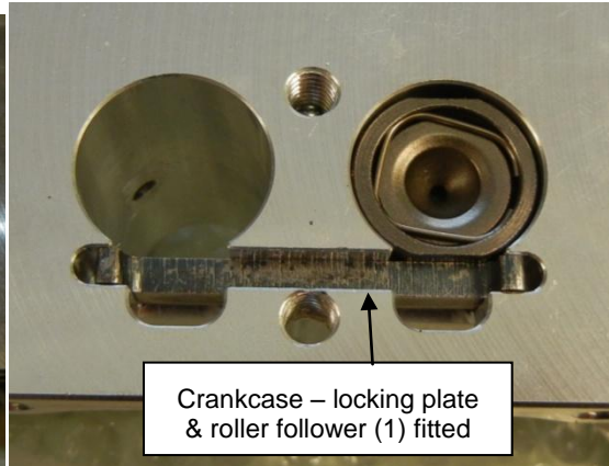
Figure 176 – Fitting Hydraulic Lifter To Crankcase
