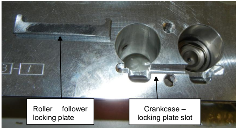
Figure 177 – Crankcase & Locking Plate
