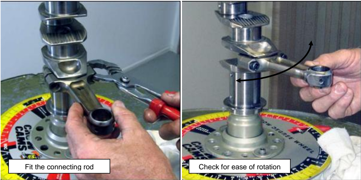
Figure 119 – Fit Connecting Rods
