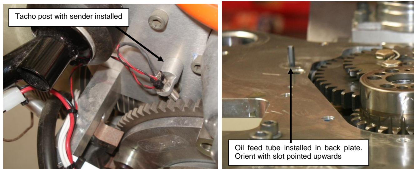
Figure 145 – Installation of Oil Feed Tubes & Tacho Pickup Post
