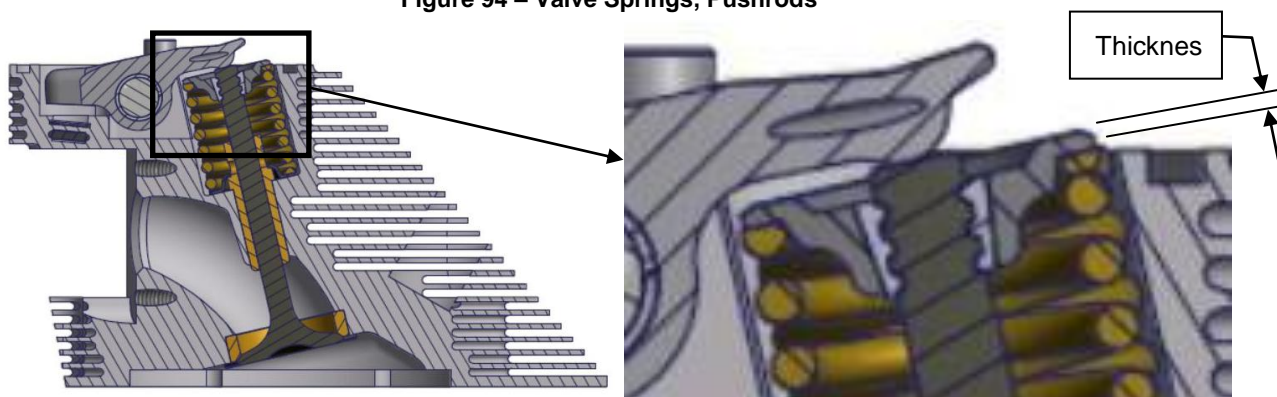
Figure 95 – Valve Spring Washer Thickness
