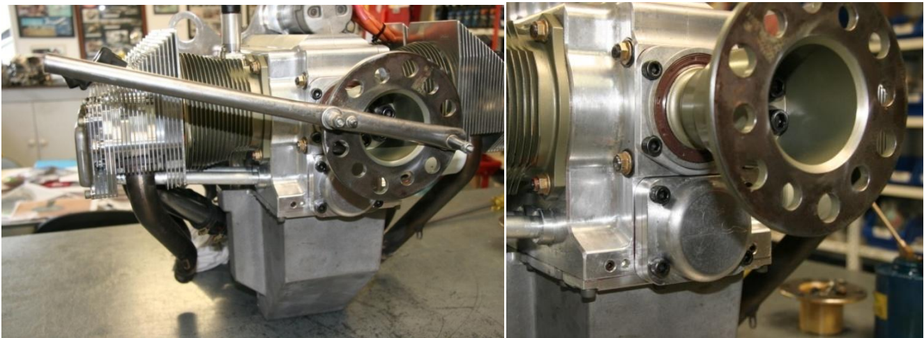
Figure 196 – Engine Turning Tool, Installed Oil Pump
