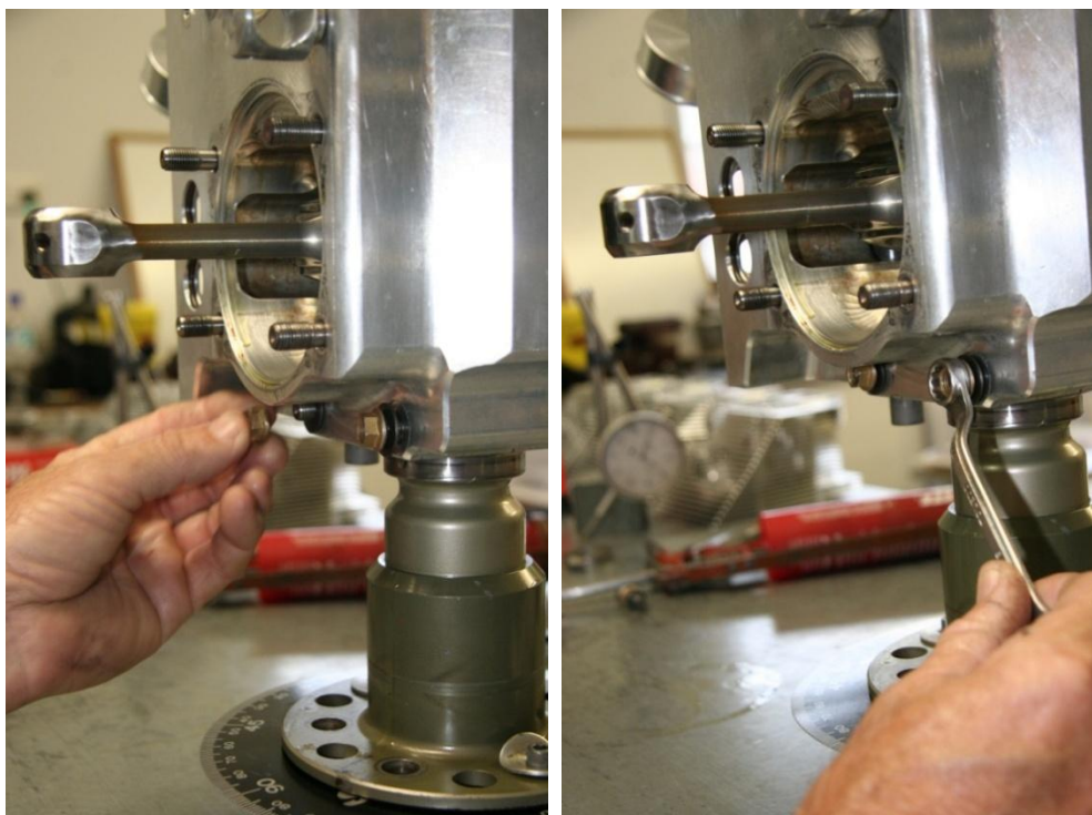
Figure 152 – Tightening The Front Crankcase Studs
