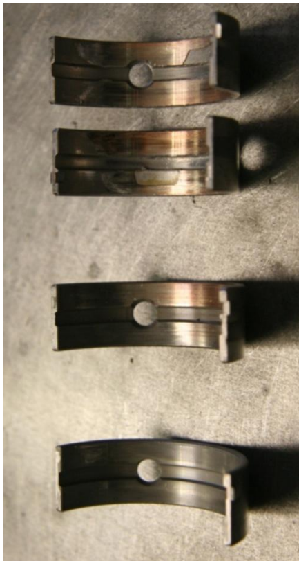
Figure 73 – Main Bearings
