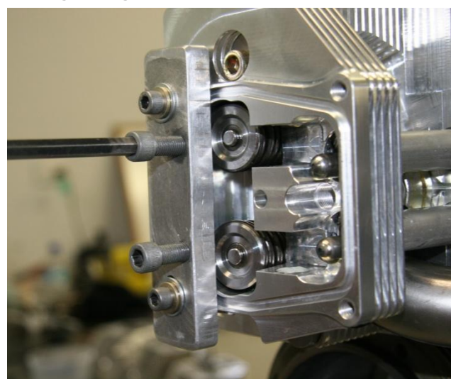
Figure 180 – Fitting Rockers #1
