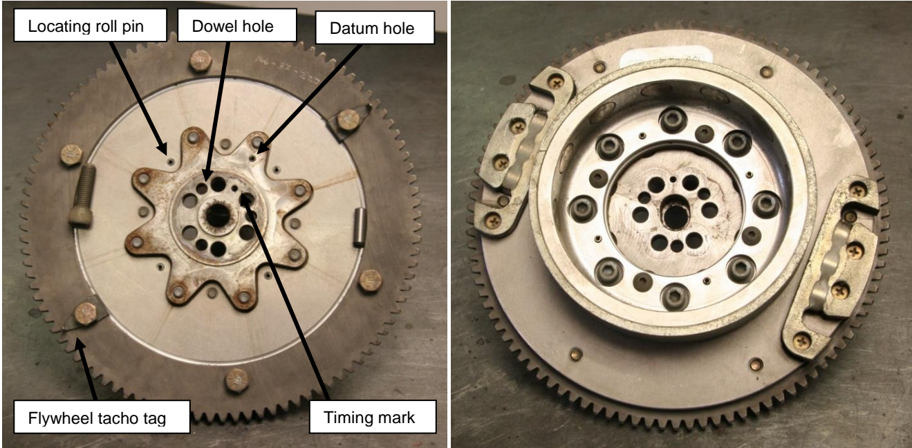
Figure 144 – Flywheel Assembly
