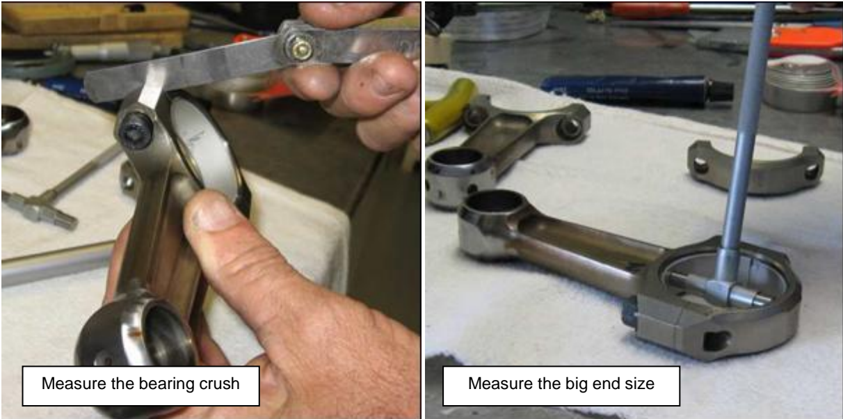
Figure 117 – Measuring Connecting Rods
