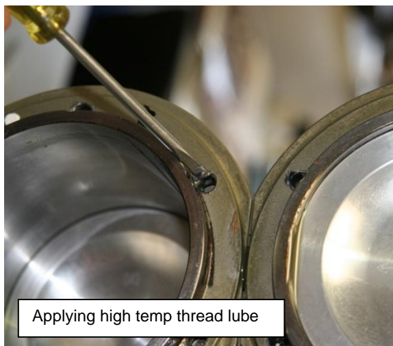
Figure 179 – Applying Thread Lubricant &amp; Tightening Lower Head Screw
