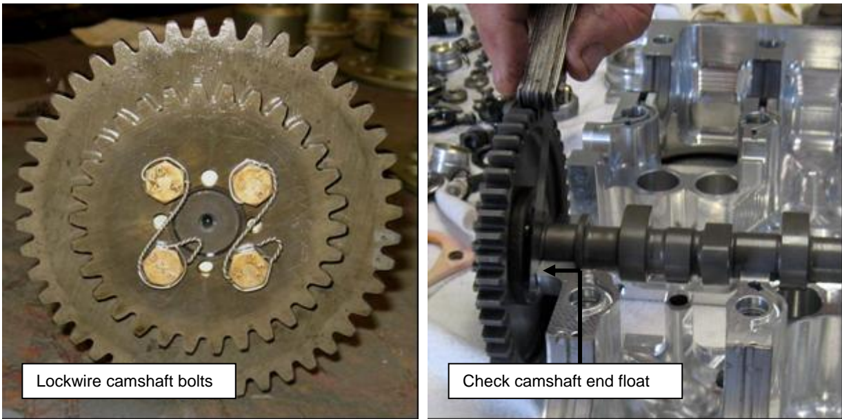
Figure 127 – Assembling Cam & Fitting to Crankcase
