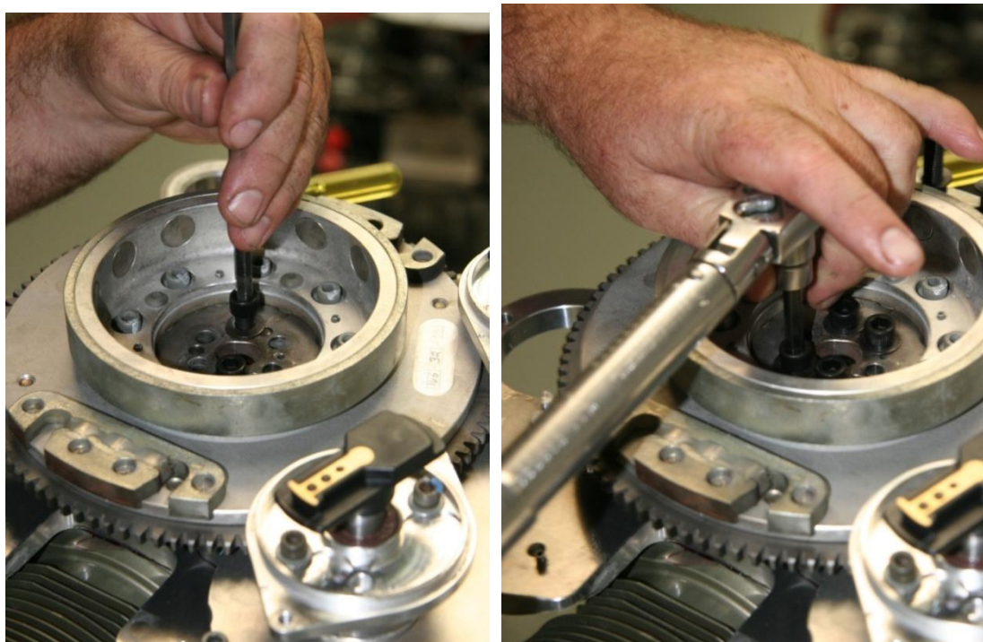
Figure 173 – Fitting &amp; Tightening Flywheel Cap Screws
