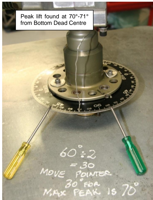
Figure 161 – Checking Cam Timing #2
