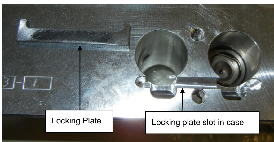
Figure 57 – Crankcase & Locking Plate
