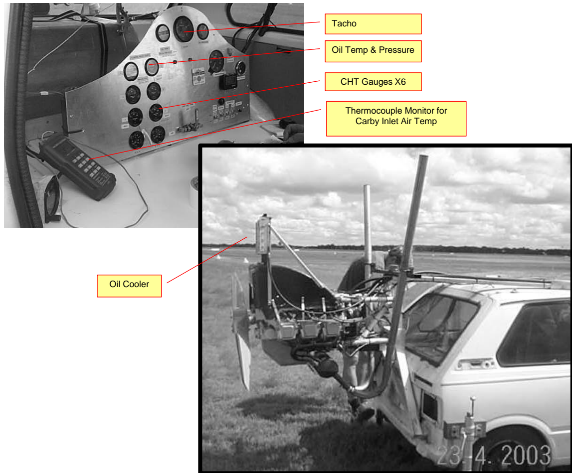
Figure 199 – Engine Ground Running Rig
