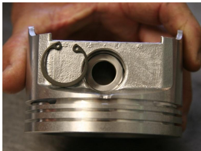
Figure 129 – Fitting Circlip to Piston
