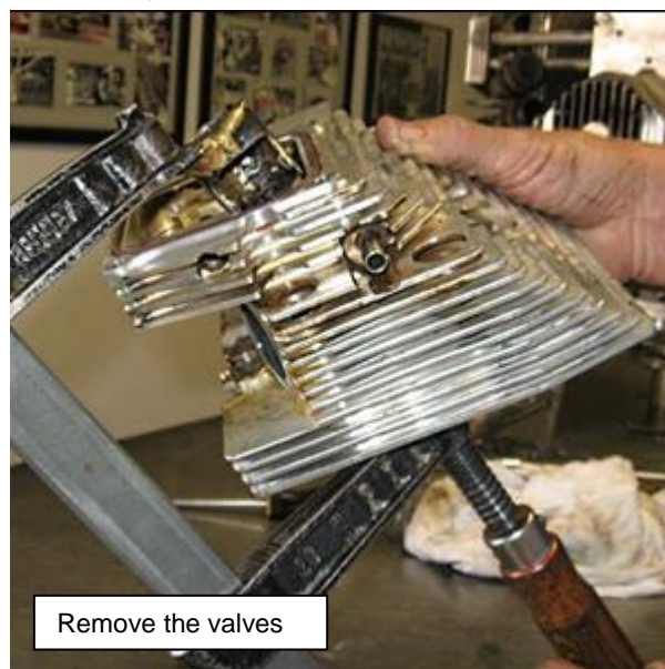
Figure 46 – Cylinder Head Disassembly
