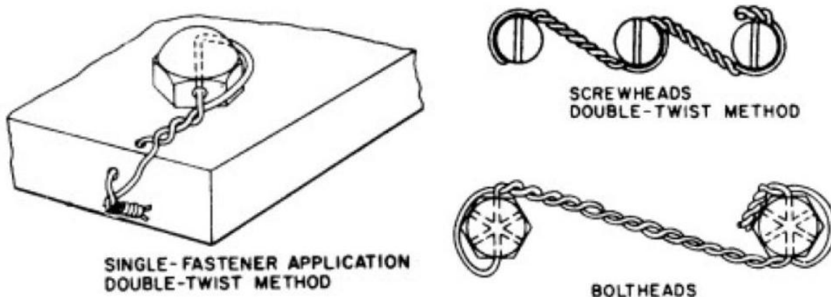
Figure 42 – Safety Wire Details
