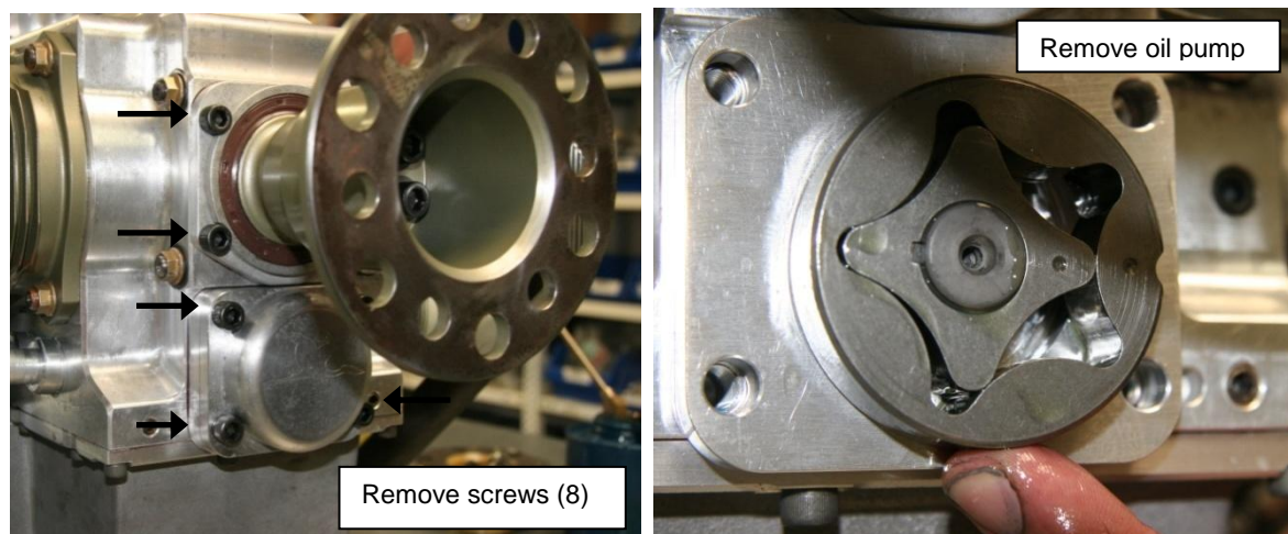
Figure 55 – Front Seal &amp; Oil Pump Removal
