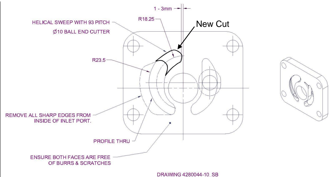
Figure 79 – Modified Port Details
