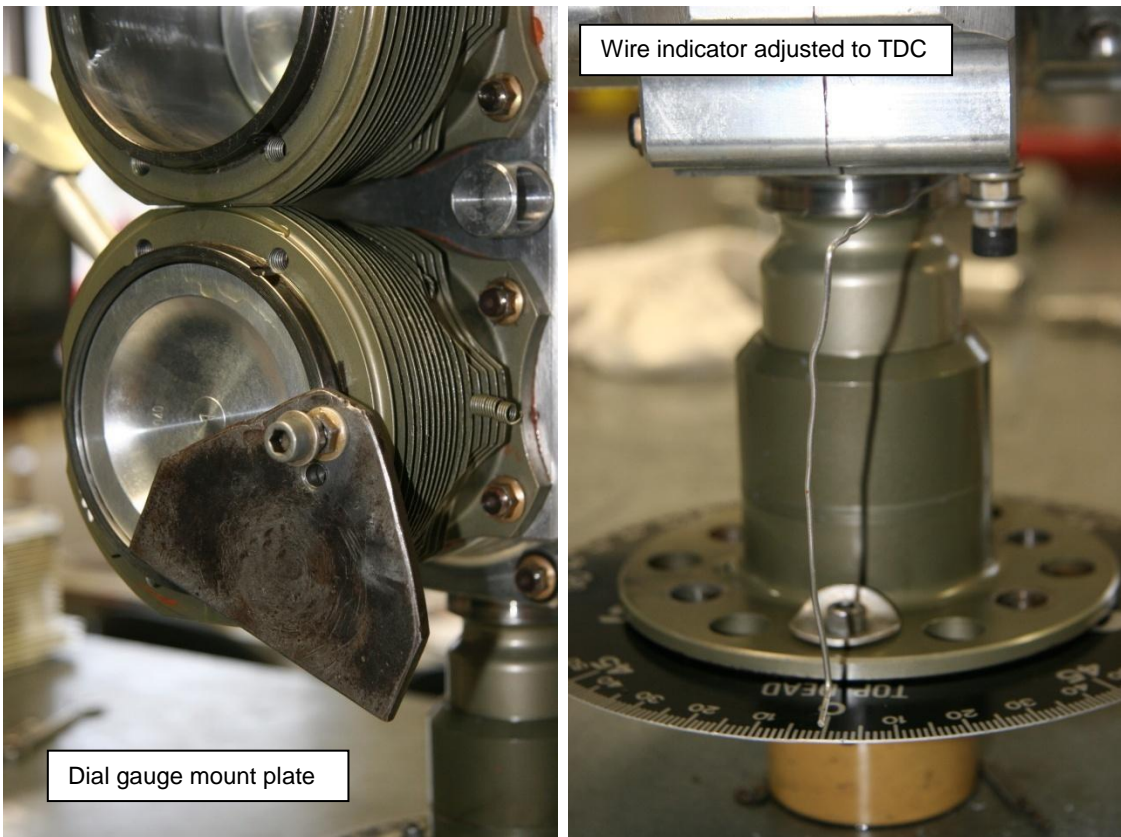
Figure 158 – Measuring Top Dead Centre
