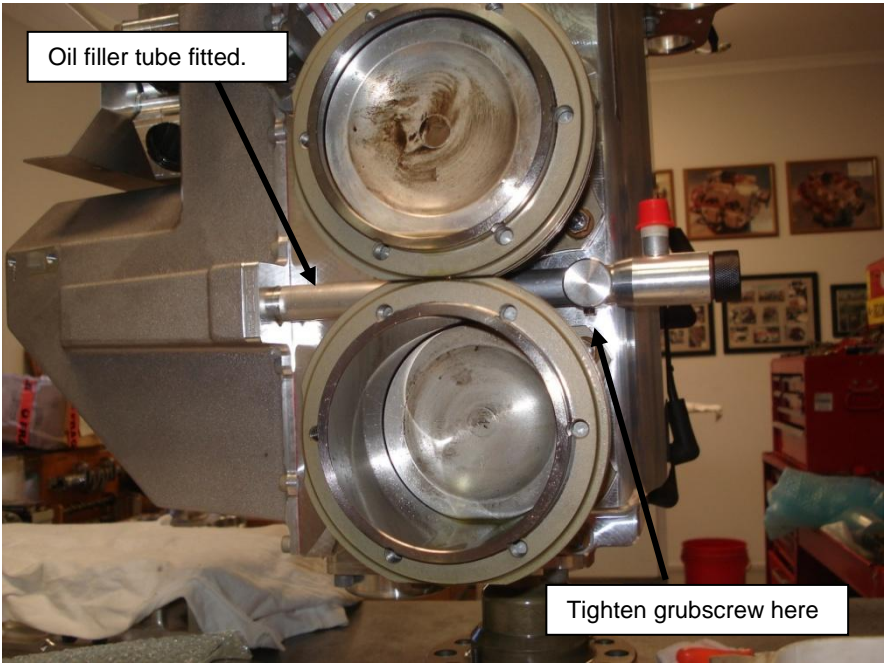
Figure 163 – Oil Filler Tube Installation
