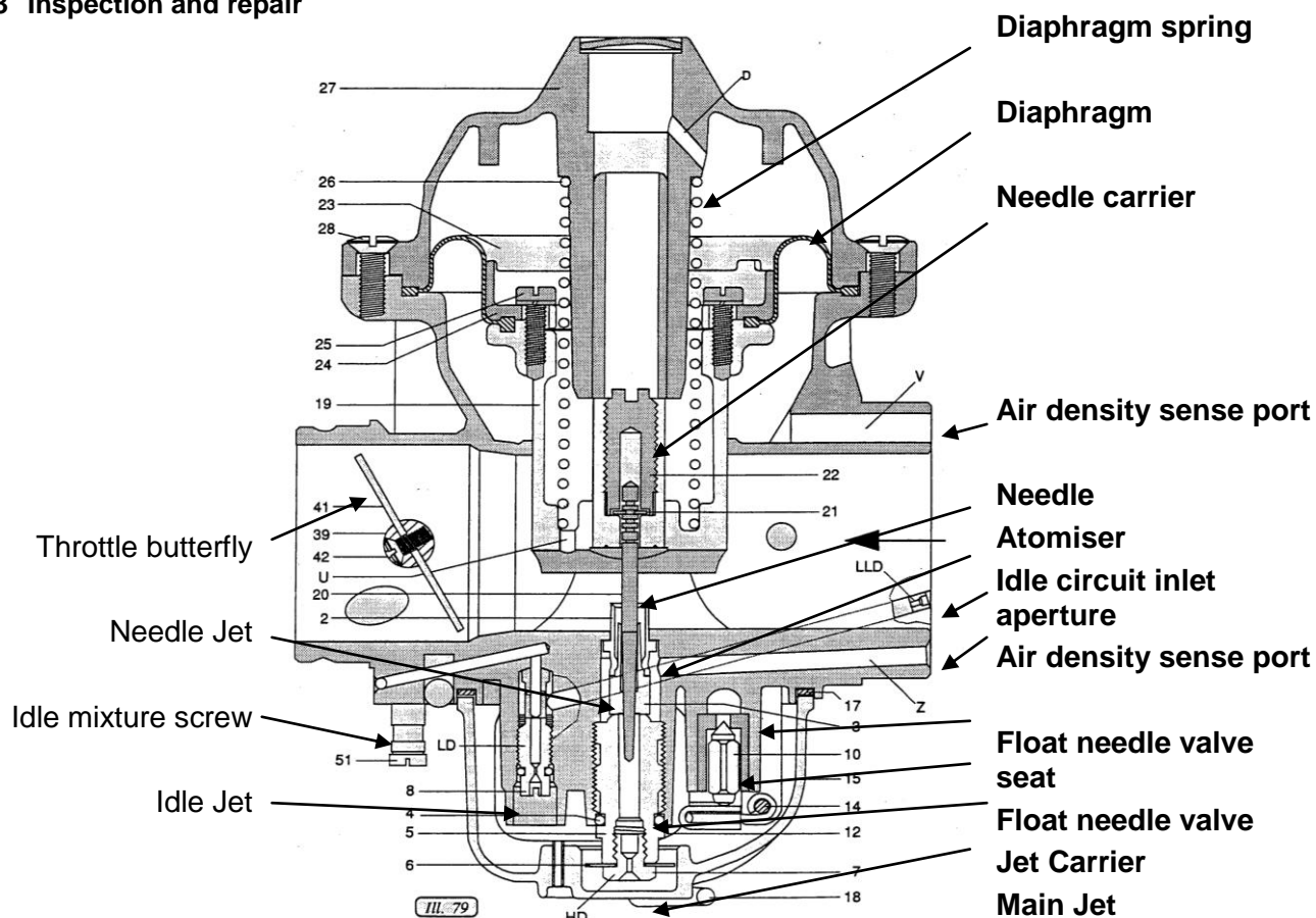
Figure 109 – Carburettor Schematic
