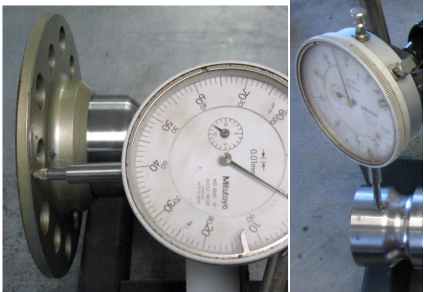
Figure 45 – Measuring Propeller Flange & Crank Run-Out
