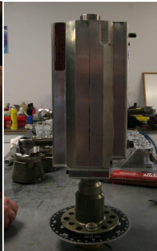
Figure 151 – Fitting The Second Case Half
