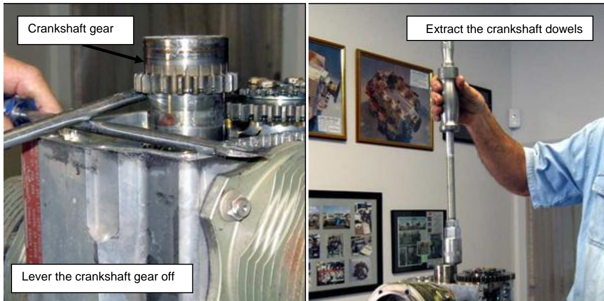
Figure 52 – Removing Crankshaft Timing Gear & Dowels
