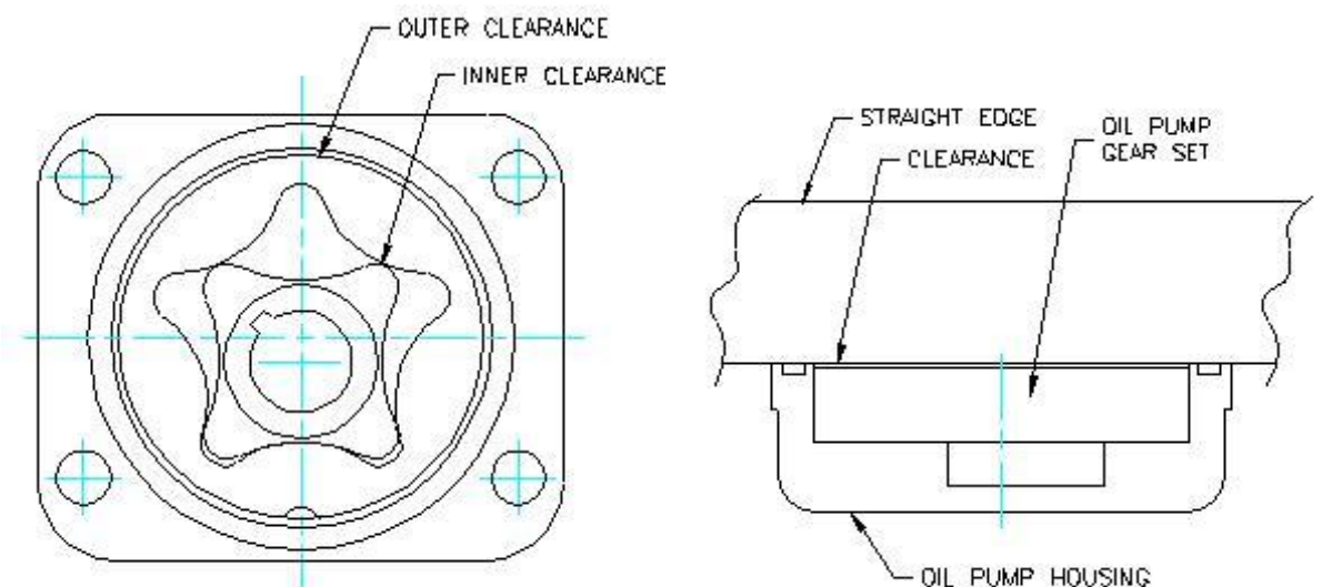
Drawing 9440064/1 OIL PUMP CLEARANCES Drawing 9428064/1 OIL PUMP END CLEARANCE Figure 200 – Oil Pump Details
