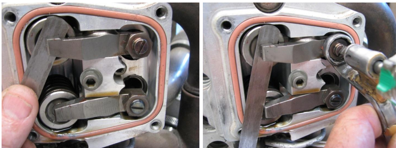
Figure 184 – Valve Clearance Adjustment (Solid Lifter)
