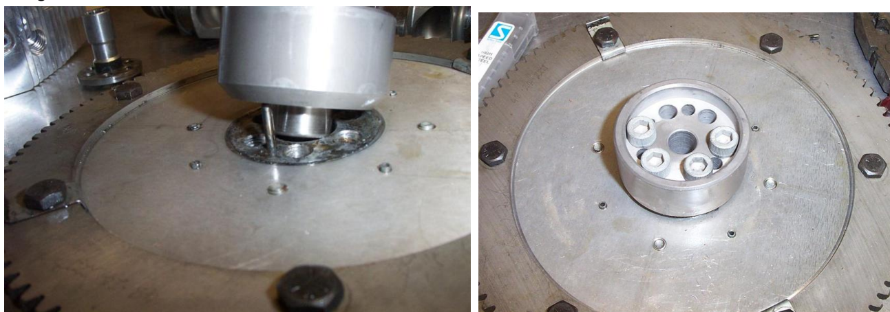
Figure 209 – Aligning Guide & Fitting To Flywheel.
