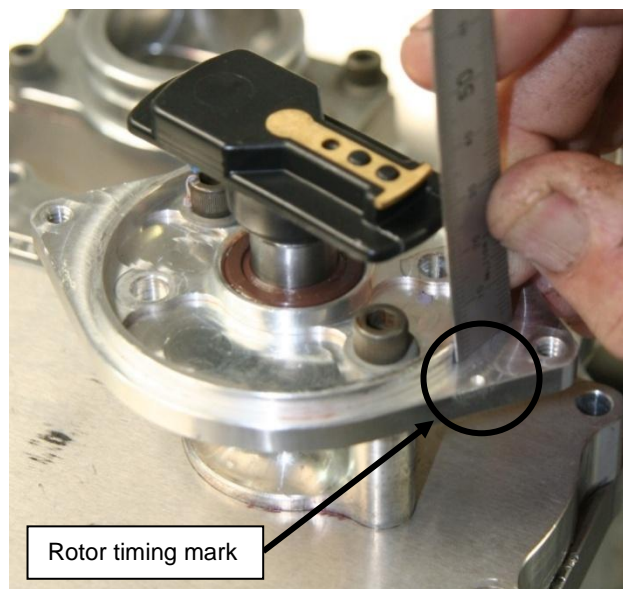
Figure 168 – Setting Distributors, Checking Rotor Position
