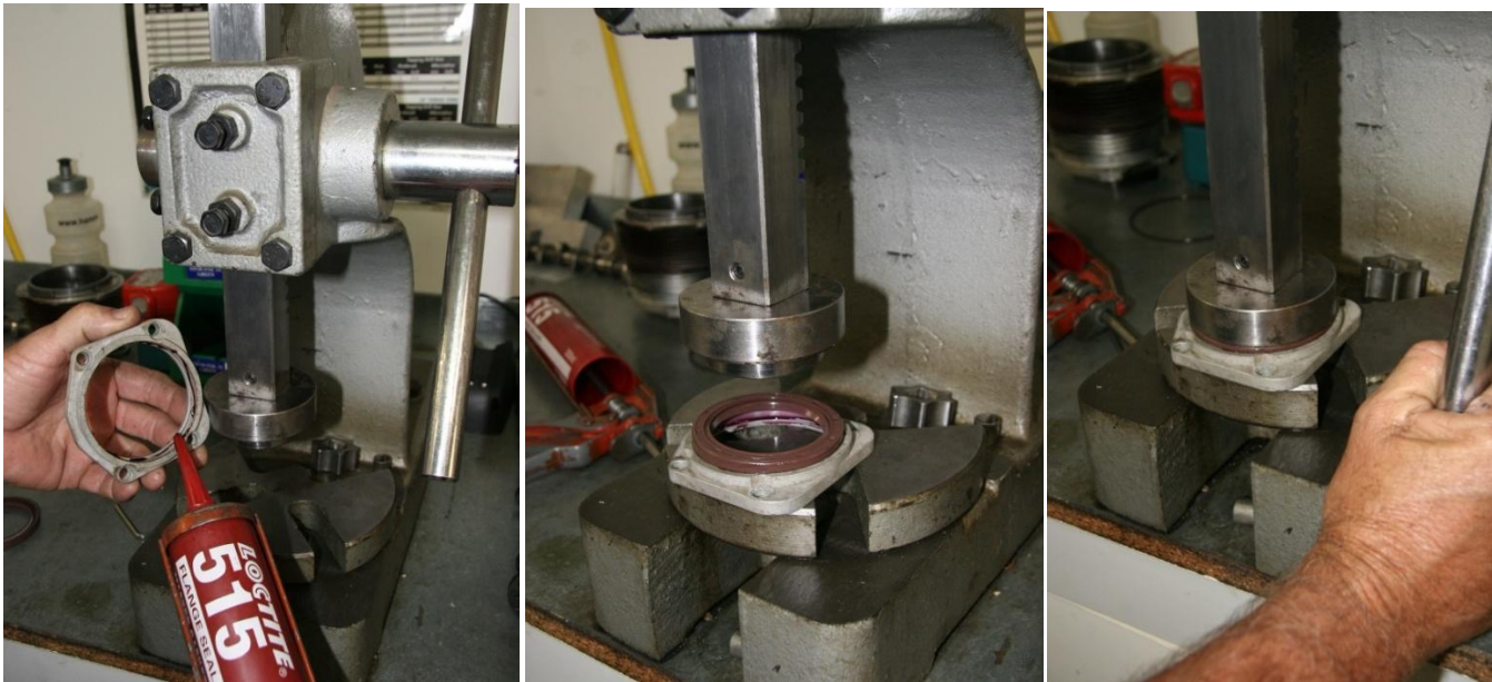
Figure 191 – Fitting Seal To Housing
