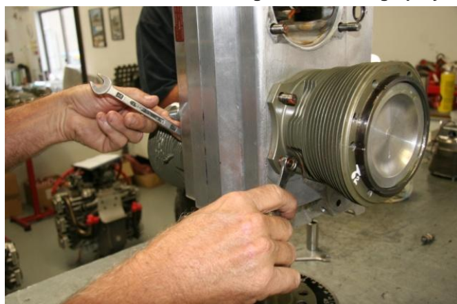
Figure 155 – Tightening Through Bolts With Lock Nuts
