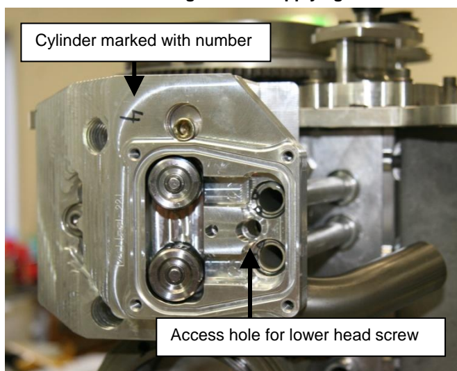
Figure 180 – Fitting Rockers #1
