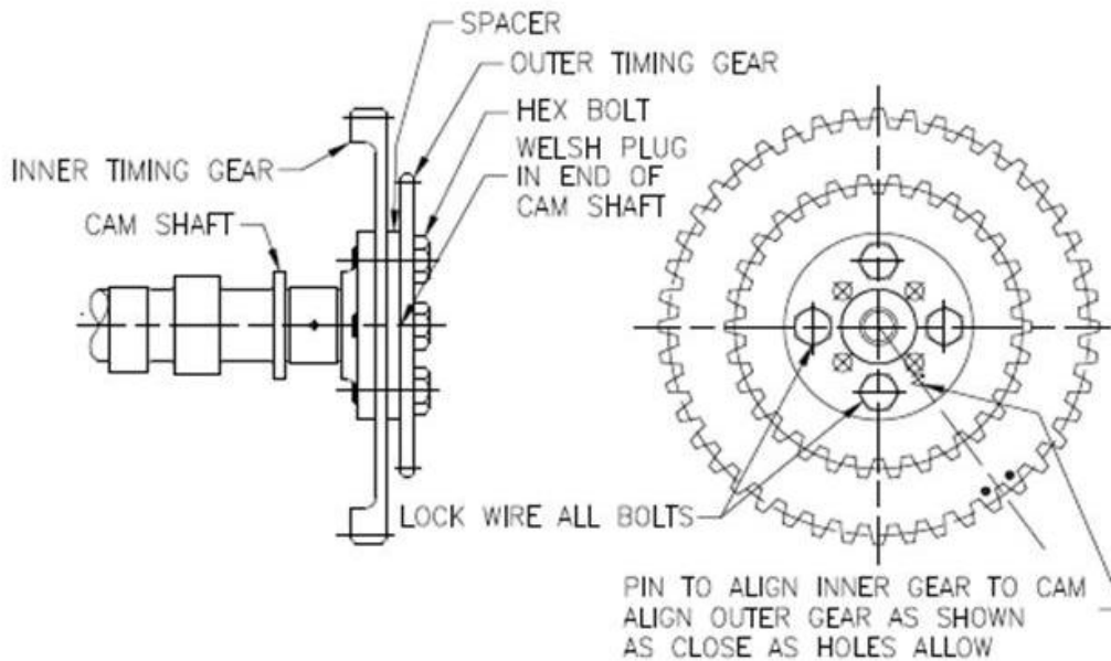
Figure 126 – Cam Timing Gear Assembly
