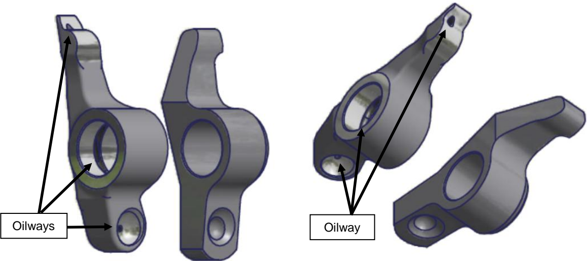
Figure 98 – Solid VS Hollow Valve Rockers
