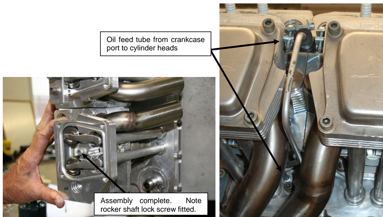
Figure 182 – Fitting Rockers #3
