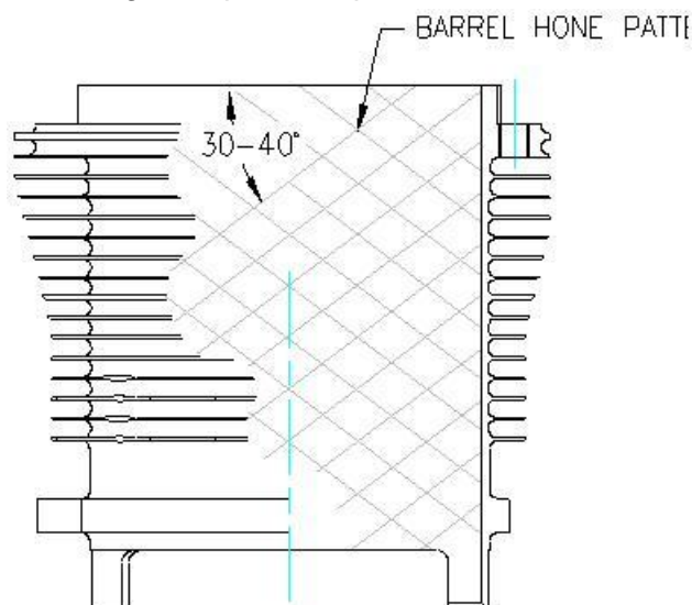
Figure 84 – Cylinder hone Pattern
