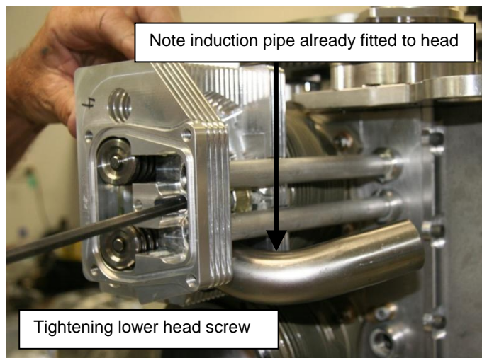
Figure 179 – Applying Thread Lubricant &amp; Tightening Lower Head Screw
