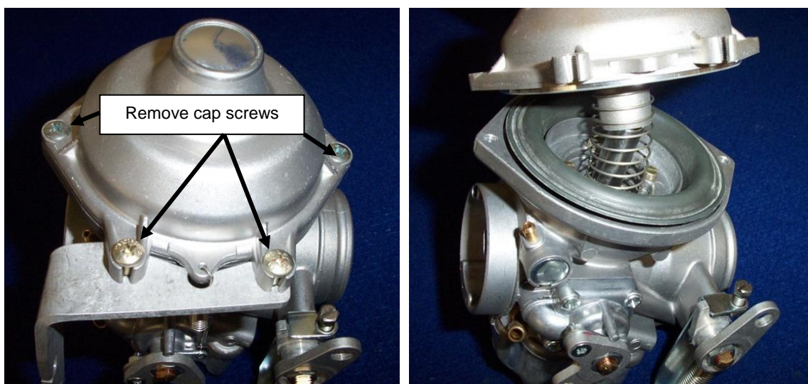
Figure 110 – Disassembling Carburettor #1
