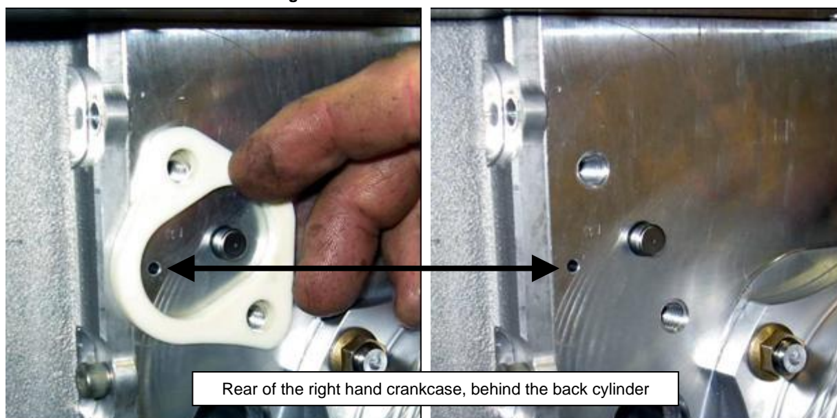
Figure 69 – Fuel Pump Oil Drain
