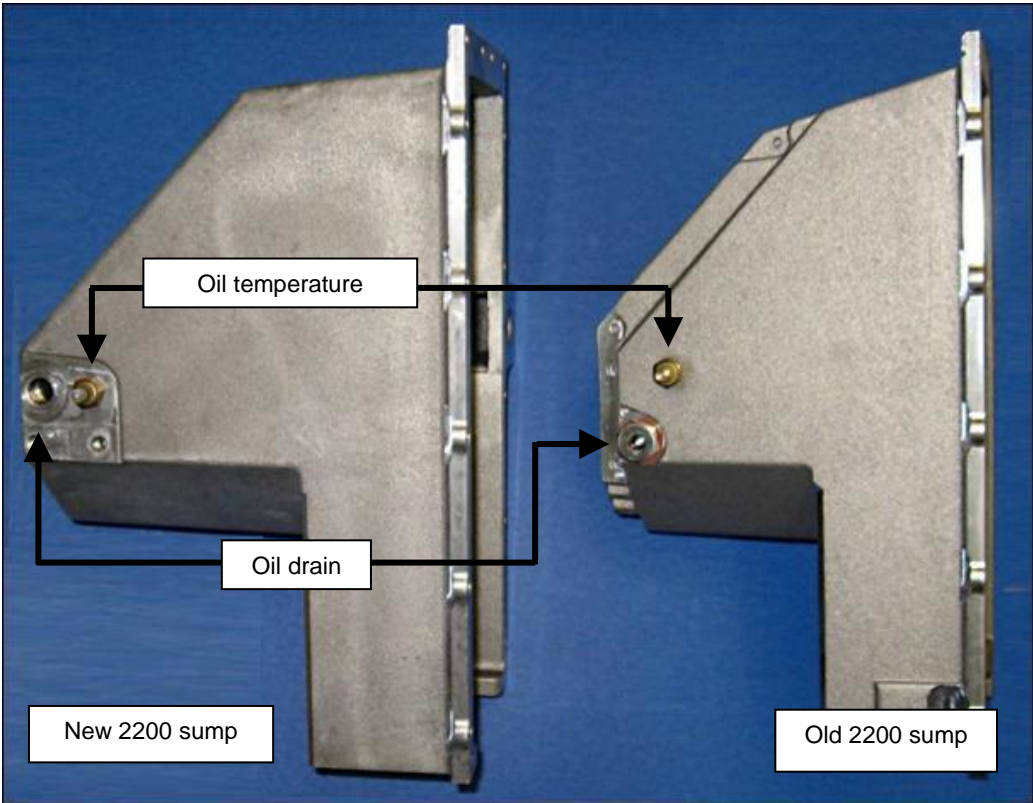
Figure 99 – 2200 Engine Sumps
