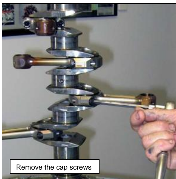
Figure 60 – Remove Con-Rods
