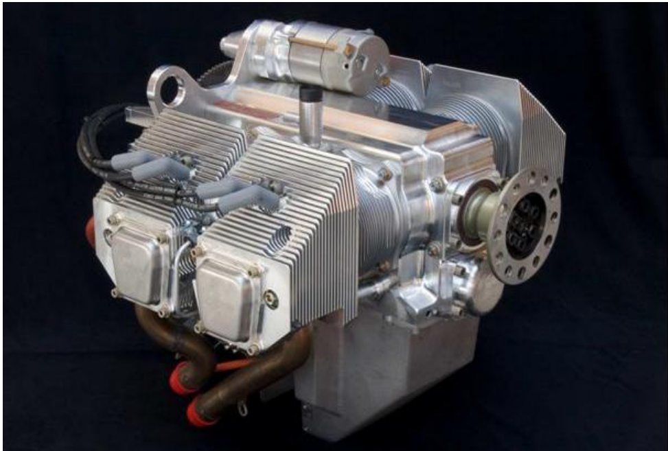
Figure 1 – 2200 Engine
