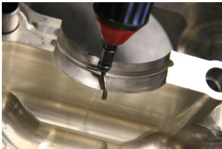
Figure 204 – De-Burring Crankcase After Surfacing & Line Boring
