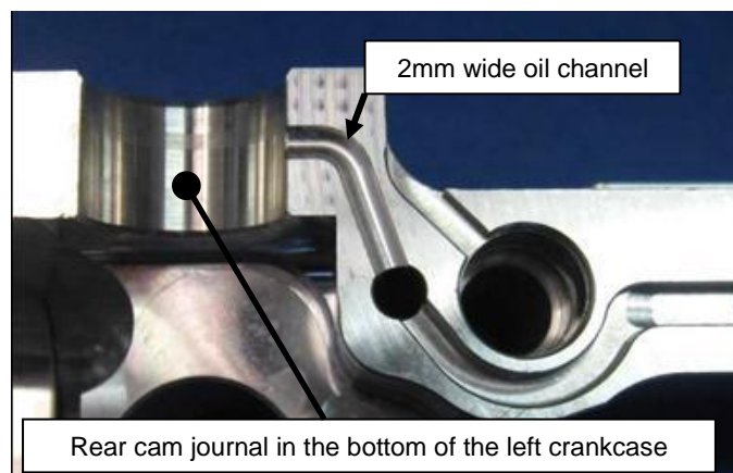
Figure 68 – Rear Cam Journal Oil Feed
