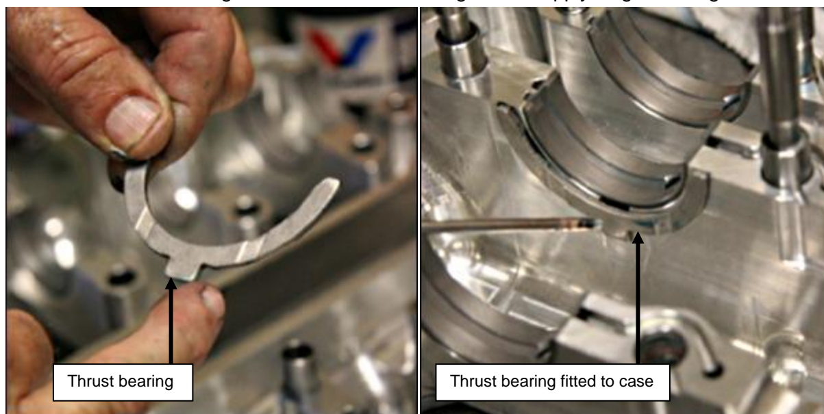
Figure 123 – Fitting Thrust Bearings
