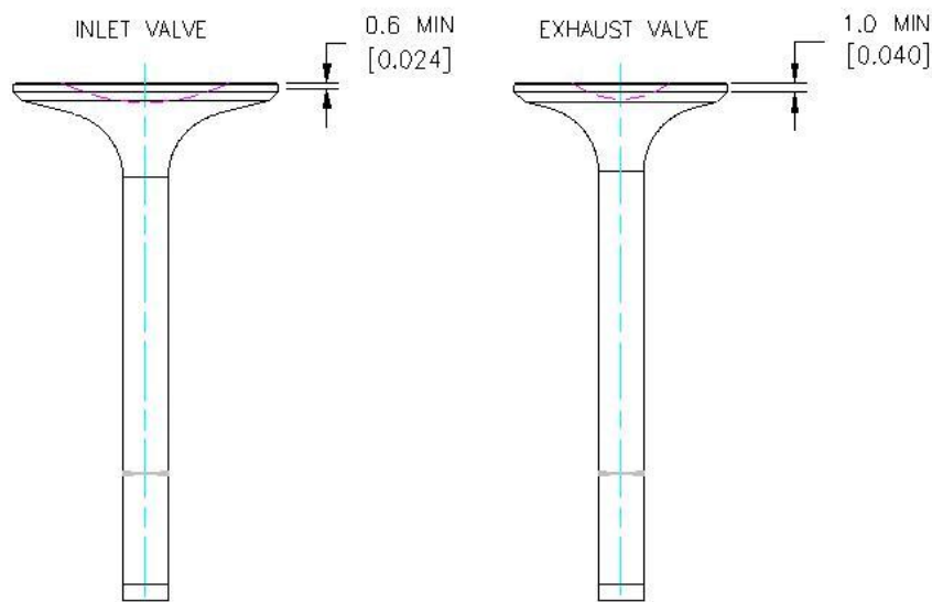
Figure 86 – Valve Measuring
