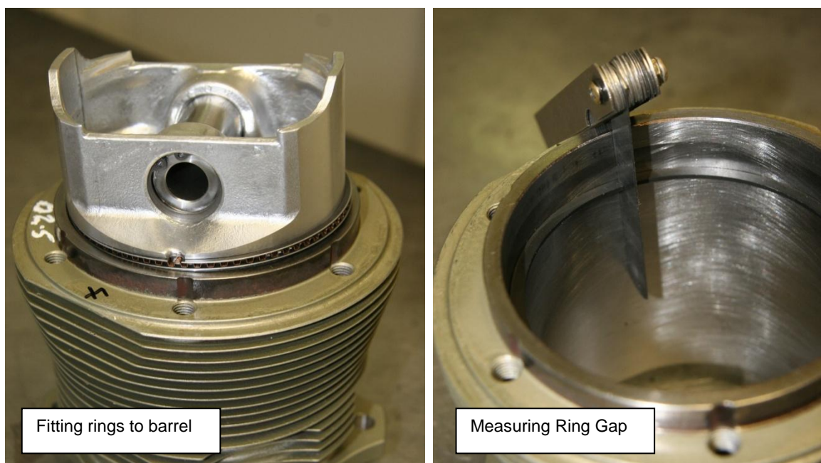
Figure 134 – Checking Piston Ring Gap
