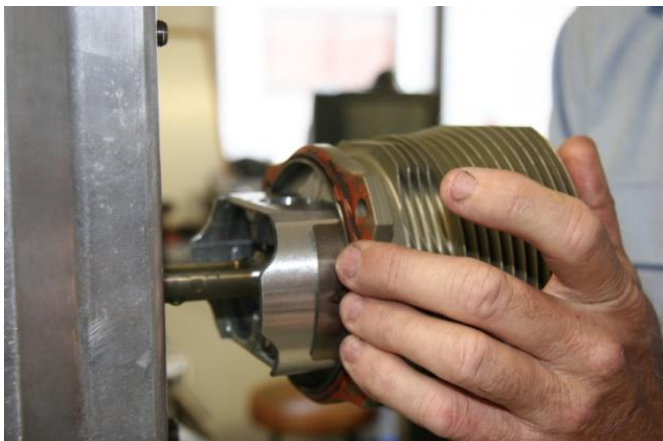
Figure 154 – Fitting Up Cylinder, Inserting Through-Bolts
