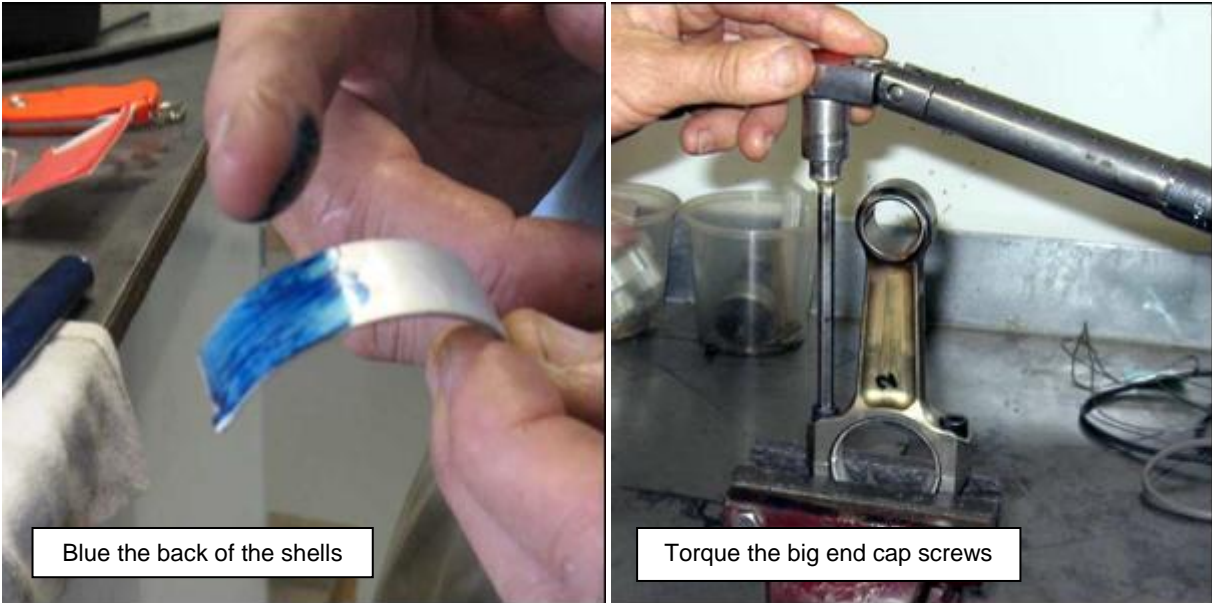
Figure 116 – Blueing Bearings, Assembling Rods
