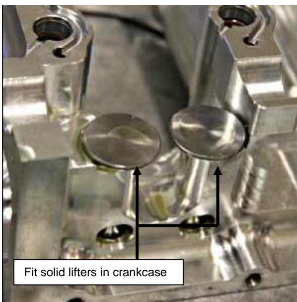
Figure 125 – Checking Crankshaft End Float, Installing Solid Lifters
