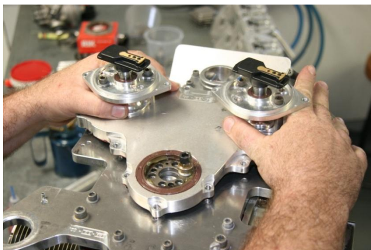
Figure 168 – Setting Distributors, Checking Rotor Position
